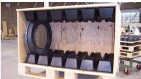
Custom Dunnage with Jet Engine Rings
